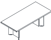
EY78 Meeting Table W:2200mm D:1000mm H:750mm
