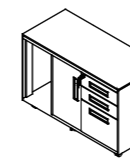
DC20.06L/R W1000*D450*H660
