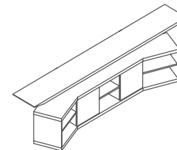
Filing Cabinet 背柜 ET92 W3250*D700*H890 (mm)
