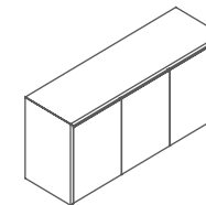
Filing Cabinet 矮柜 ET91 W1600*D480*H740 (mm)
